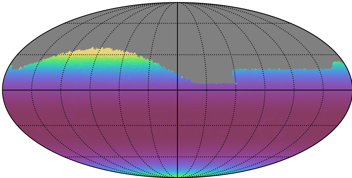
baseline_v3.3_10yrs Yr 1 all bands: Min airmass
