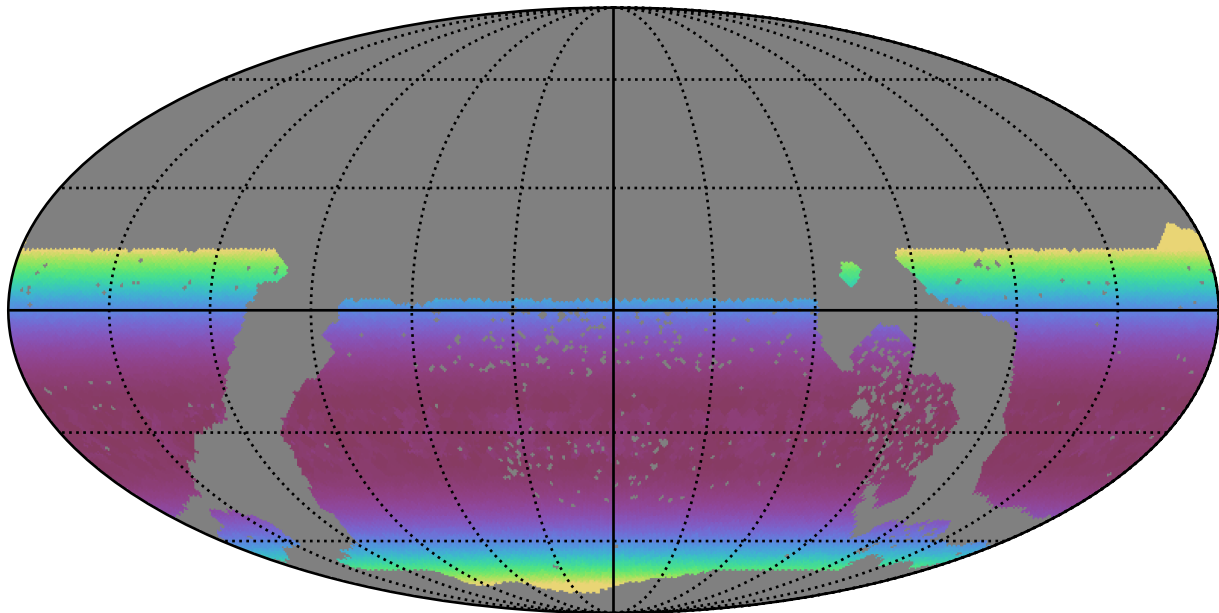
baseline_v3.3_10yrs WFD z band: Min airmass
