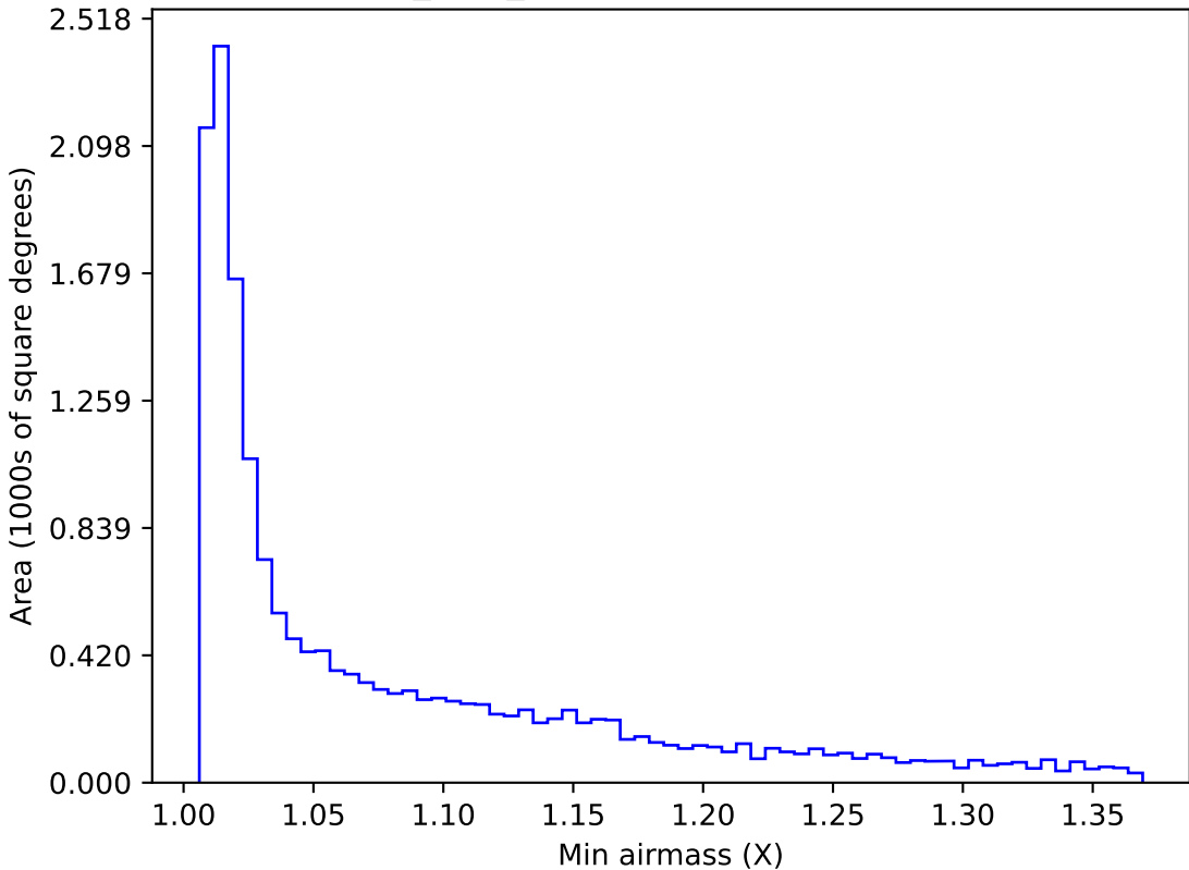
baseline_v3.3_10yrs WFD z band: Min airmass
