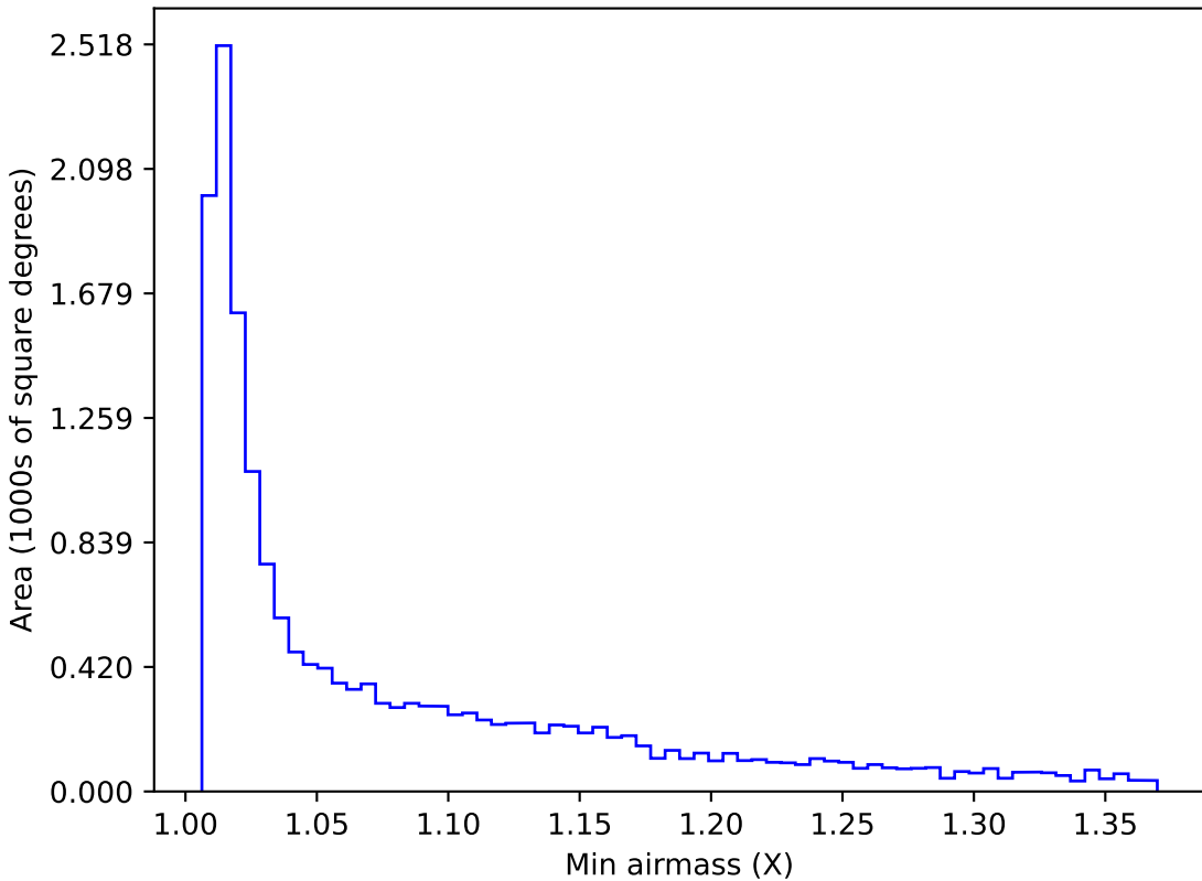
baseline_v3.3_10yrs WFD y band: Min airmass
