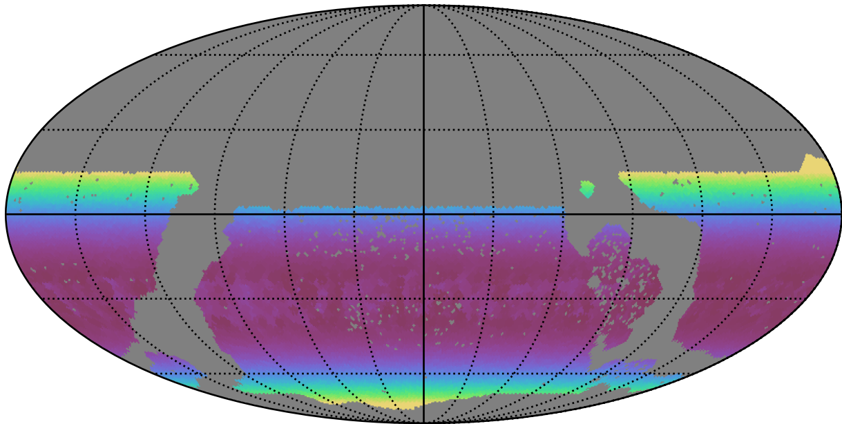
baseline_v3.3_10yrs WFD u band: Min airmass
