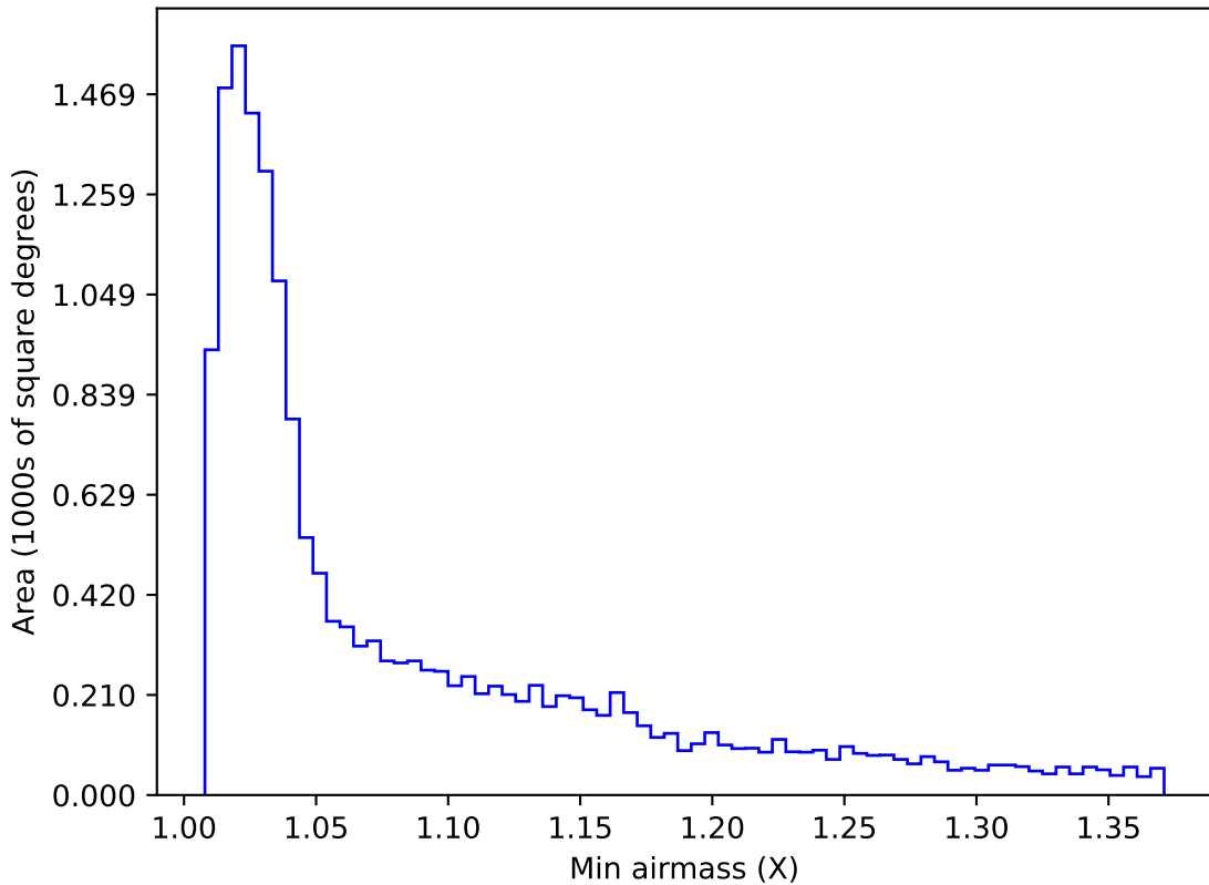
baseline_v3.3_10yrs WFD u band: Min airmass
