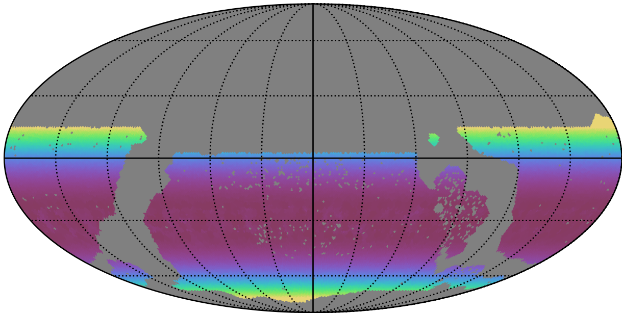
baseline_v3.3_10yrs WFD r band: Min airmass
