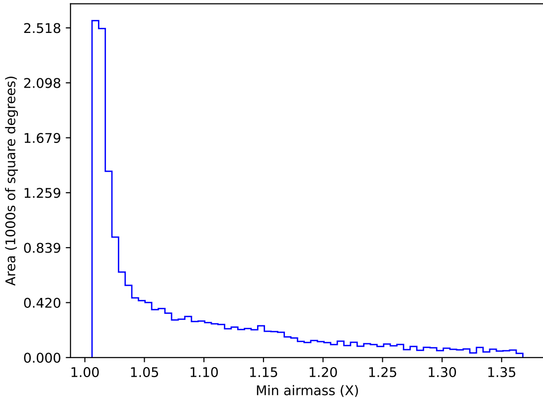
baseline_v3.3_10yrs WFD r band: Min airmass
