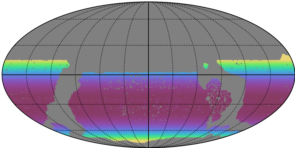
baseline_v3.3_10yrs WFD i band: Min airmass
