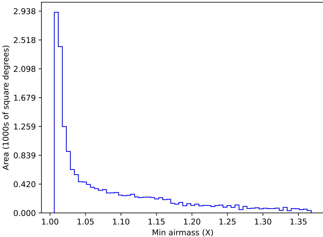
baseline_v3.3_10yrs WFD i band: Min airmass
