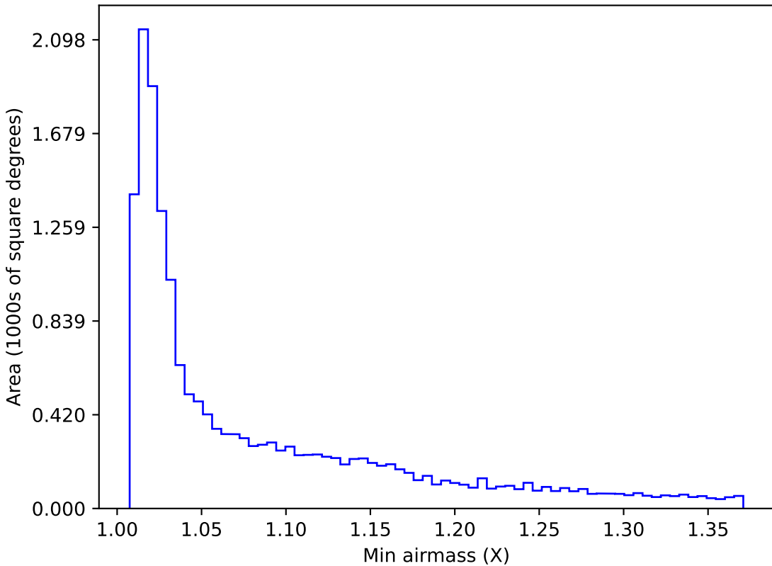
baseline_v3.3_10yrs WFD g band: Min airmass
