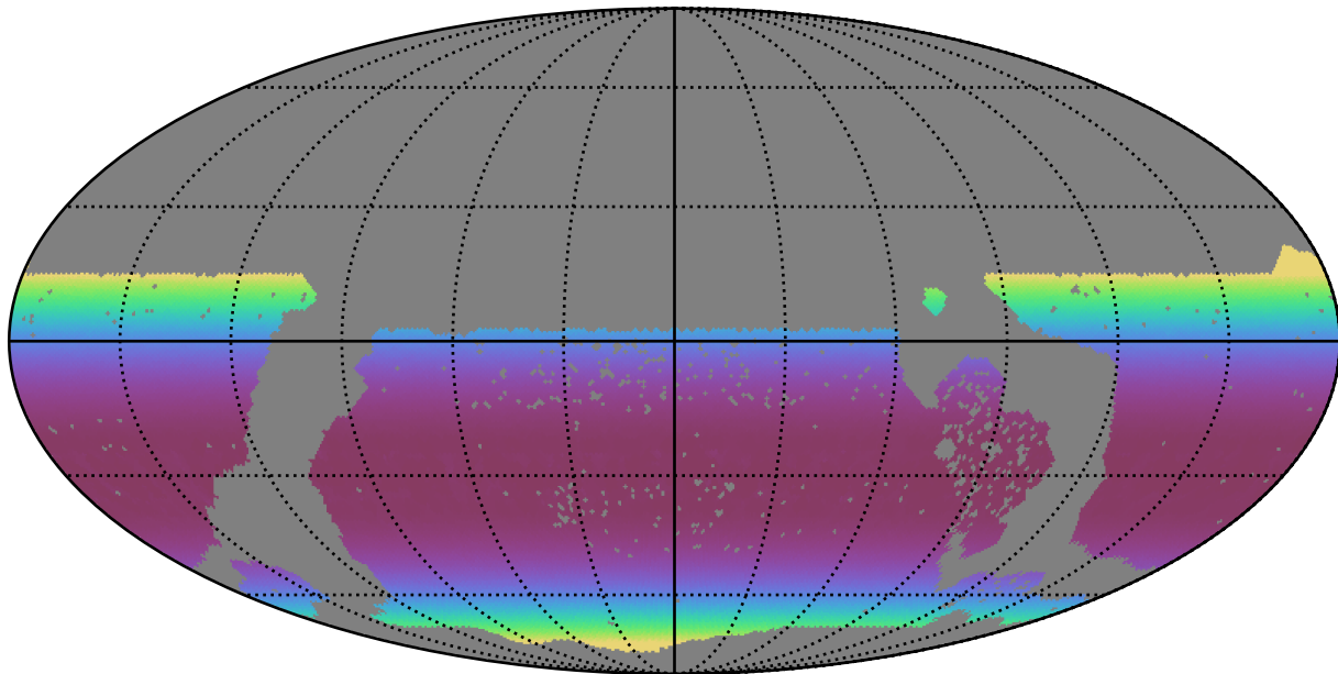
baseline_v3.3_10yrs WFD all bands: Min airmass
