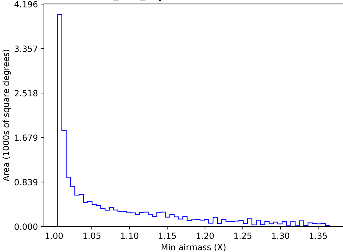
baseline_v3.3_10yrs WFD all bands: Min airmass
