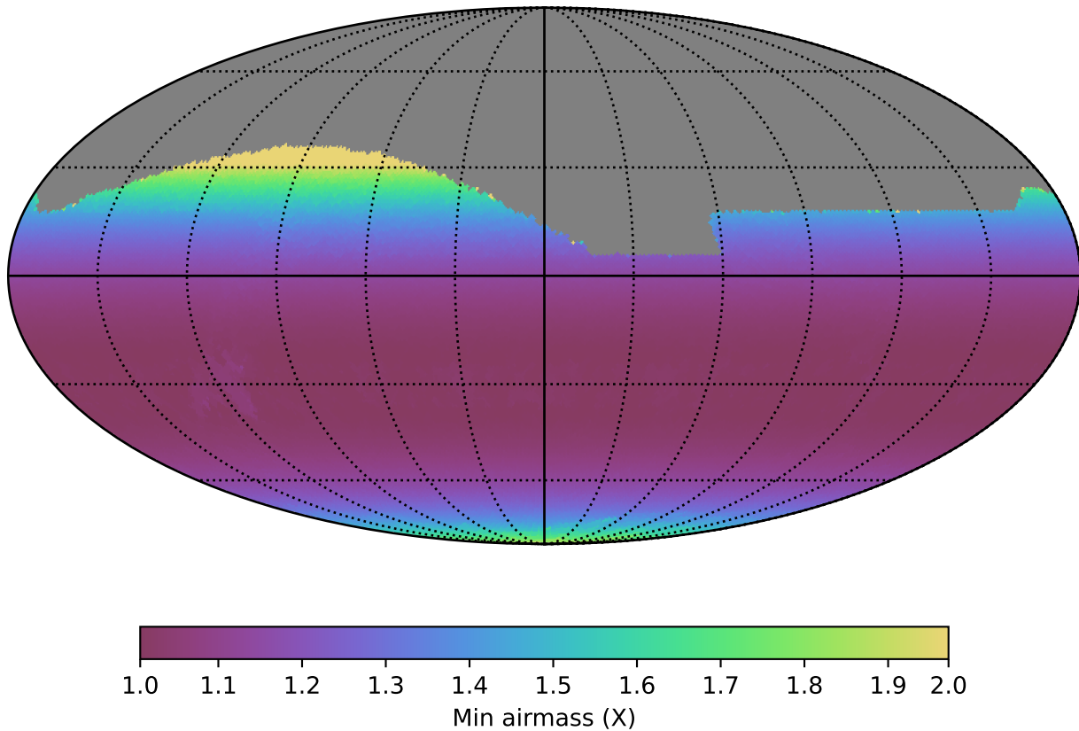
baseline_v3.3_10yrs All sky z band: Min airmass
