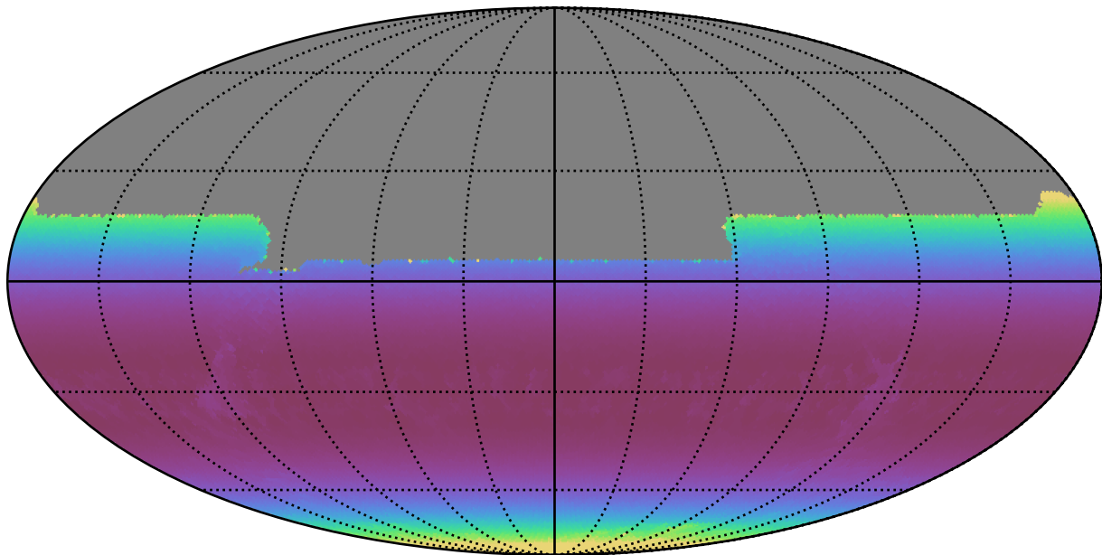
baseline_v3.3_10yrs All sky y band: Min airmass
