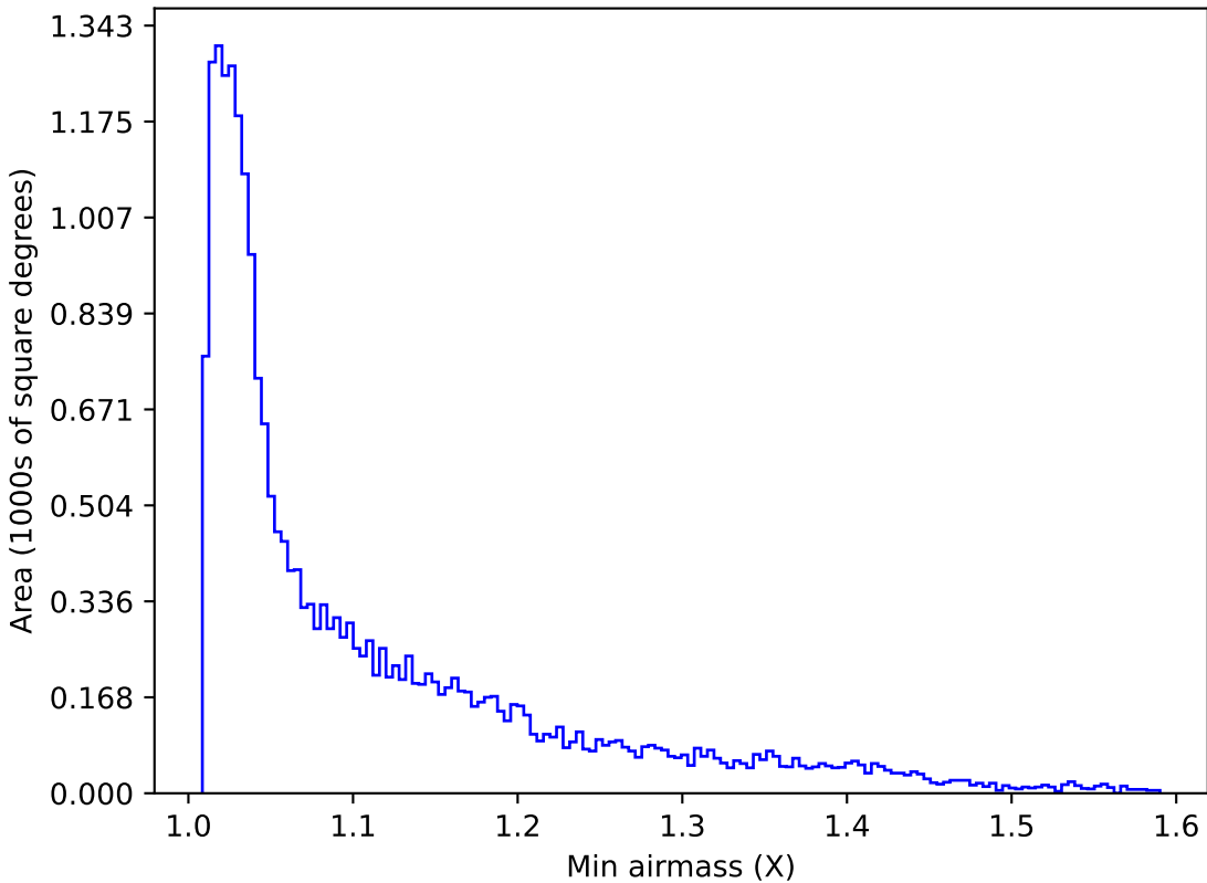
baseline_v3.3_10yrs All sky u band: Min airmass
