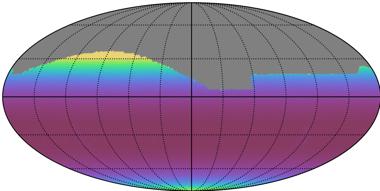
baseline_v3.3_10yrs All sky r band: Min airmass
