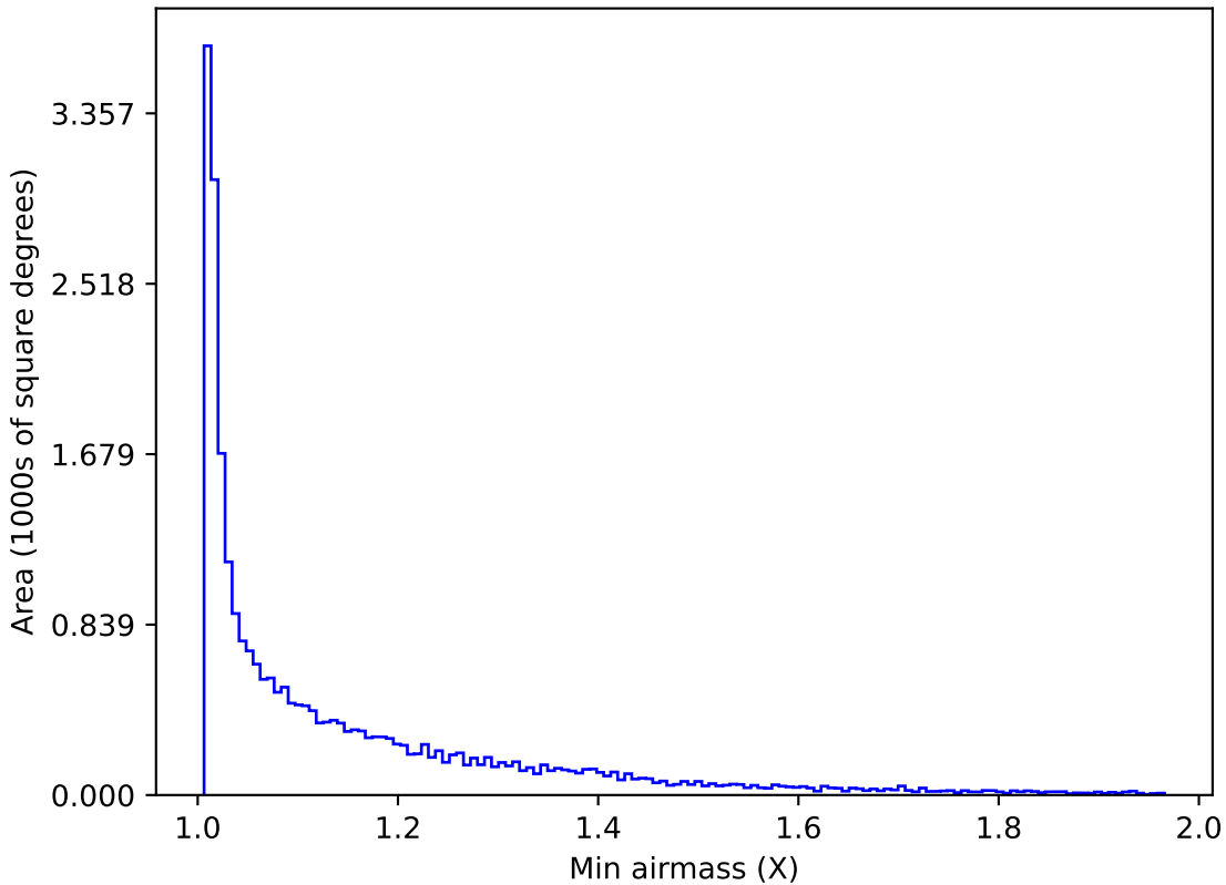
baseline_v3.3_10yrs All sky r band: Min airmass
