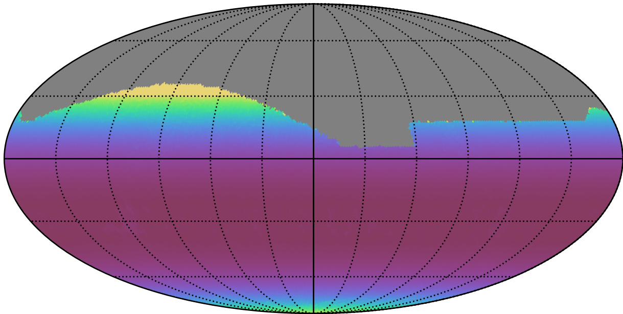
baseline_v3.3_10yrs All sky i band: Min airmass
