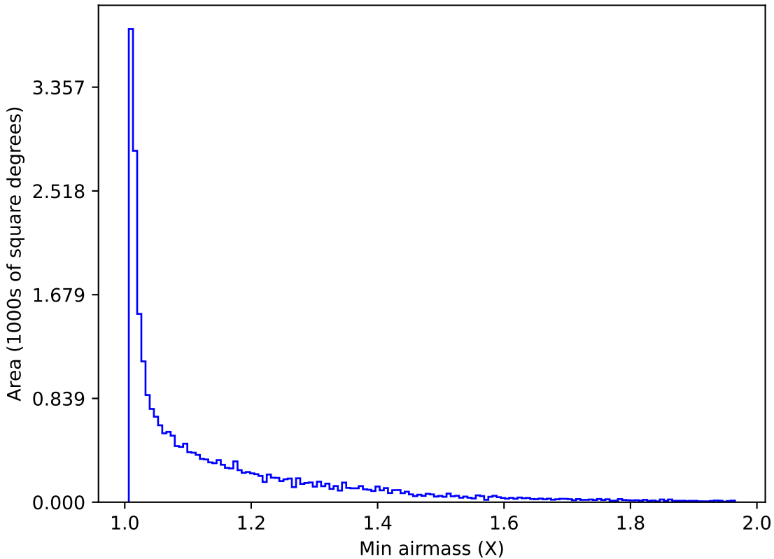
baseline_v3.3_10yrs All sky i band: Min airmass
