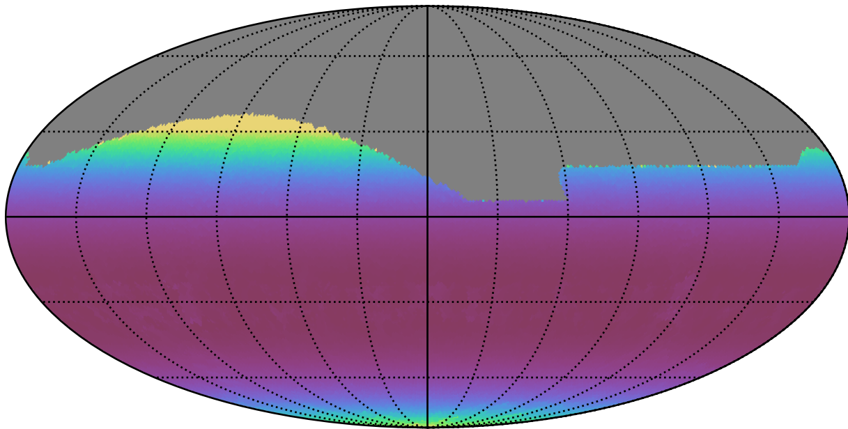
baseline_v3.3_10yrs All sky g band: Min airmass
