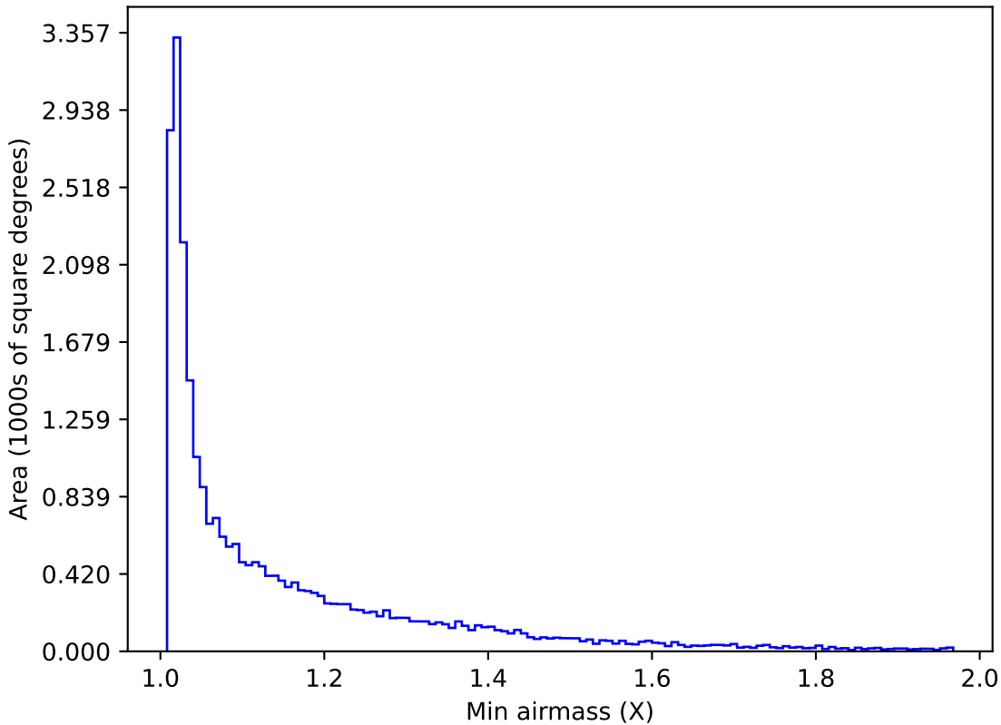
baseline_v3.3_10yrs All sky g band: Min airmass
