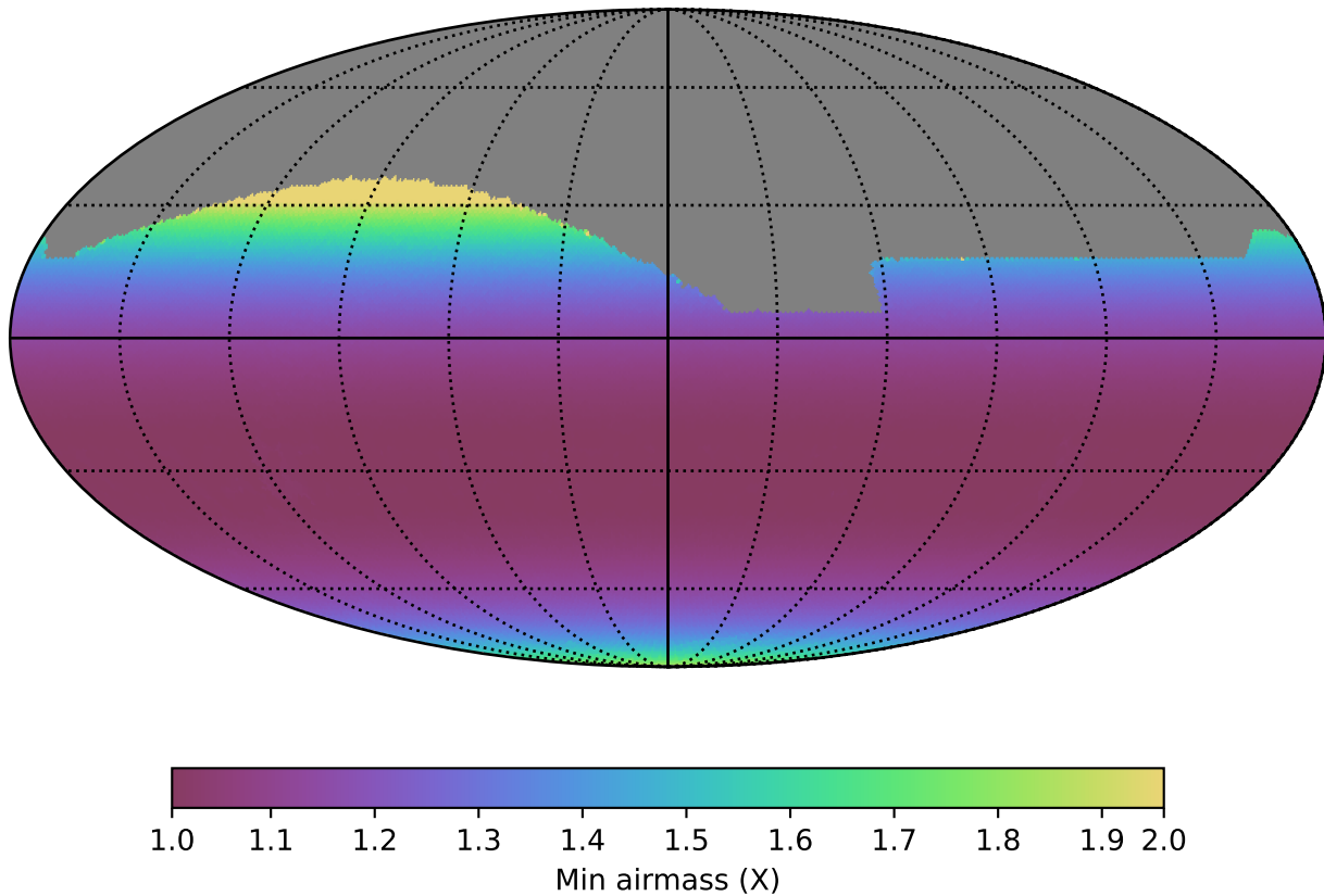
baseline_v3.3_10yrs All sky all bands: Min airmass
