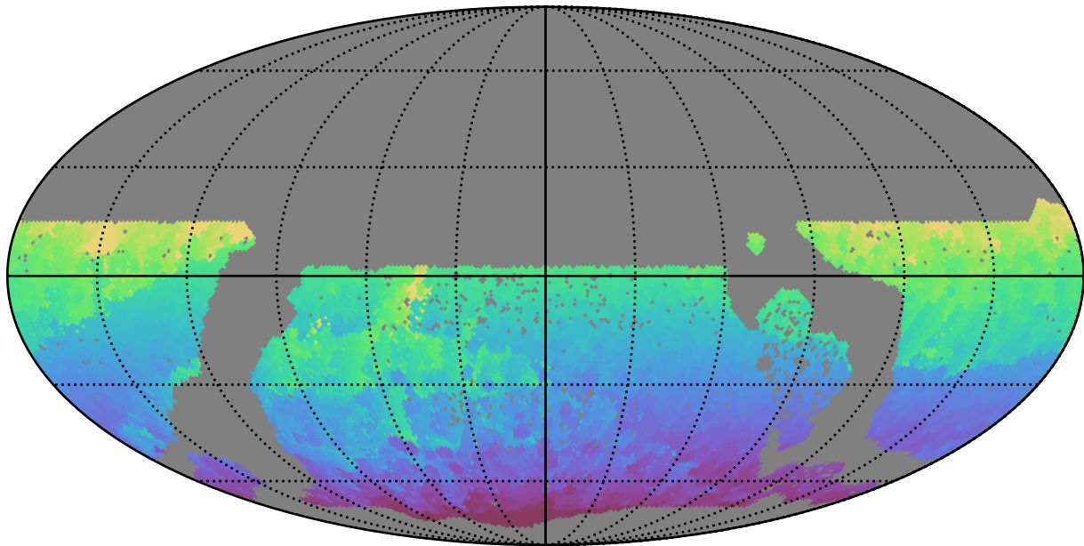
baseline_v3.3_10yrs WFD all bands: Min HA
