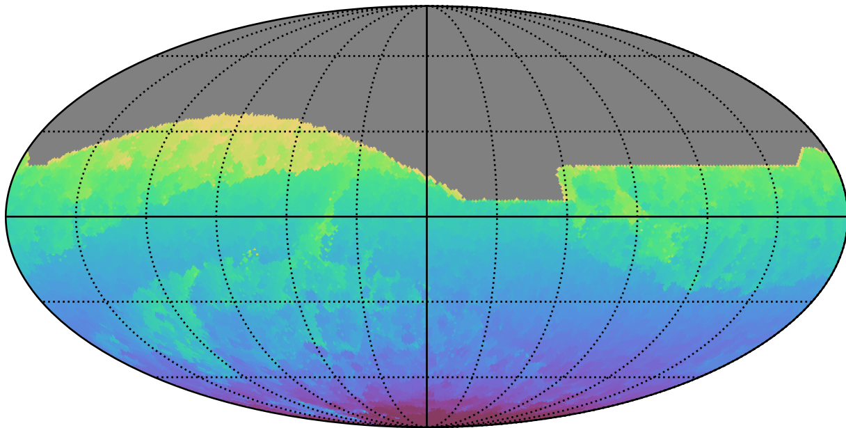
baseline_v3.3_10yrs All sky all bands: Min HA
