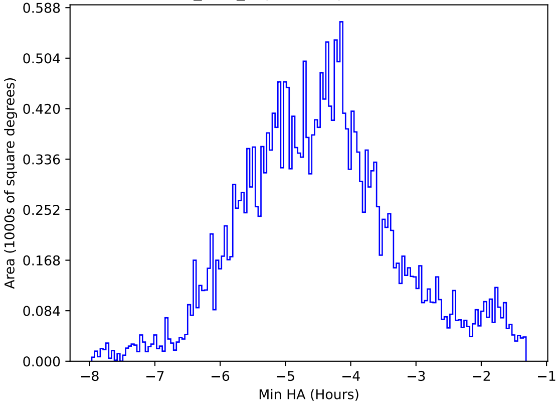
baseline_v3.3_10yrs All sky all bands: Min HA
