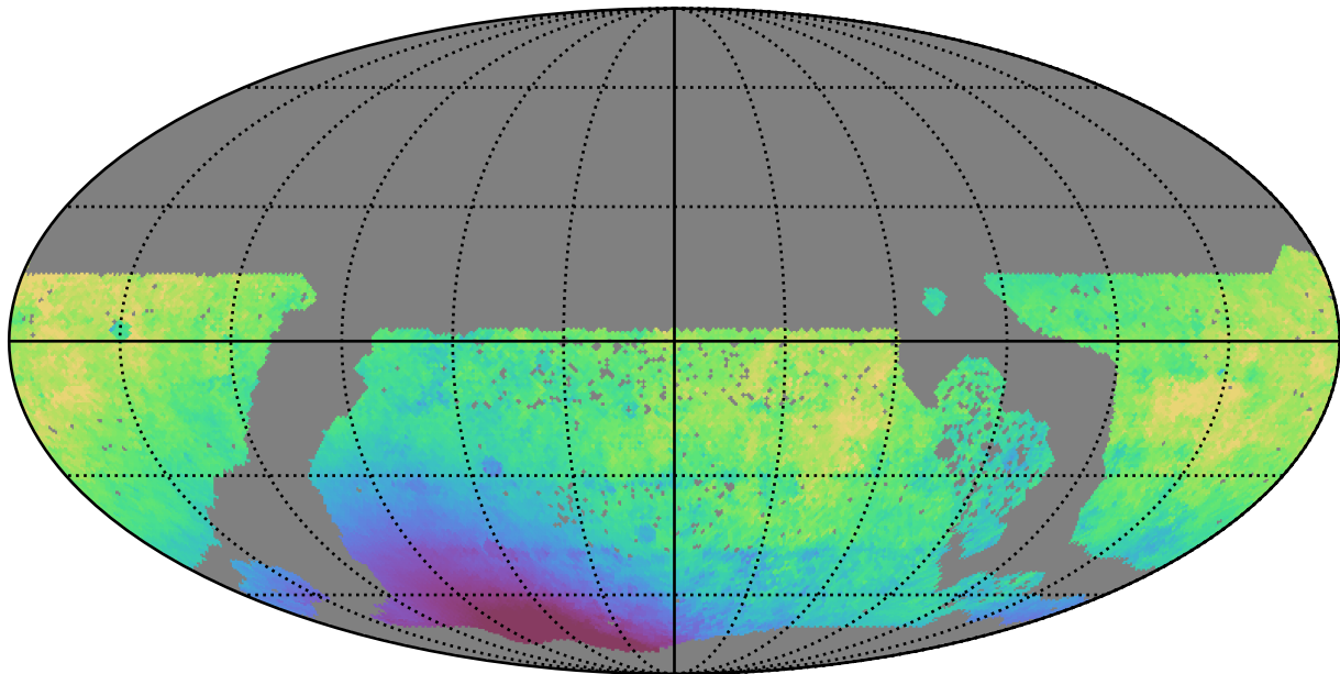
baseline_v3.3_10yrs WFD z band: Median solarElong
