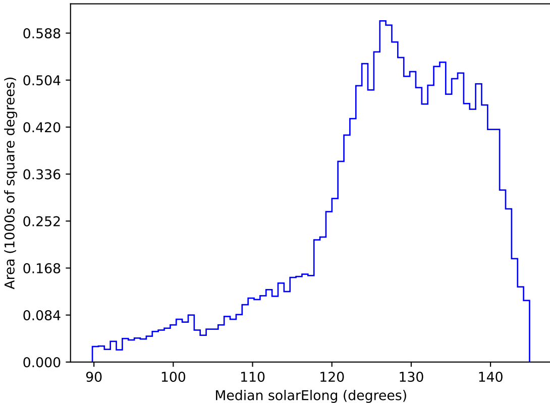
baseline_v3.3_10yrs WFD z band: Median solarElong
