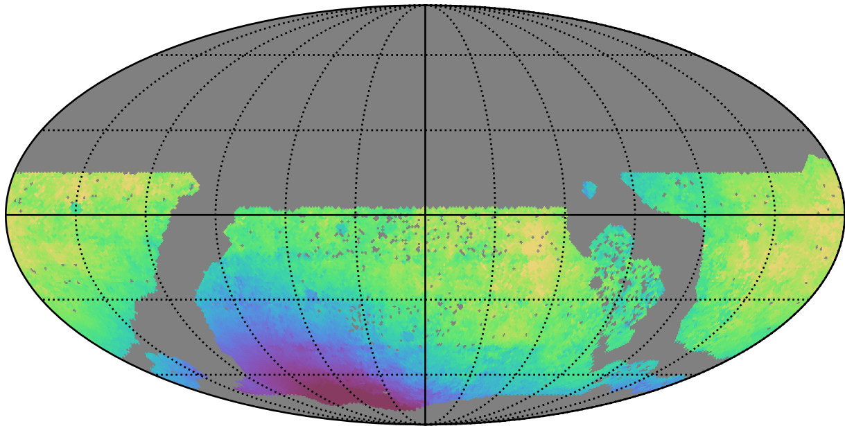
baseline_v3.3_10yrs WFD y band: Median solarElong
