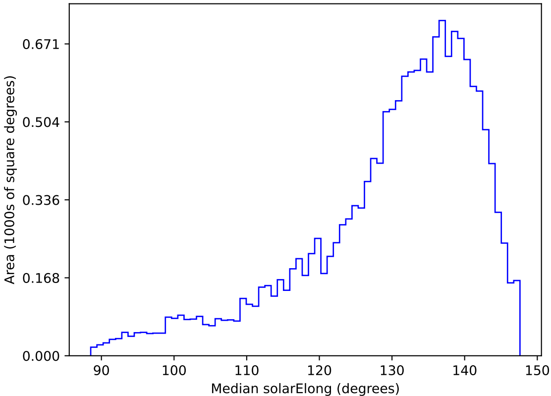
baseline_v3.3_10yrs WFD y band: Median solarElong
