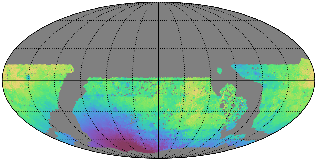
baseline_v3.3_10yrs WFD u band: Median solarElong
