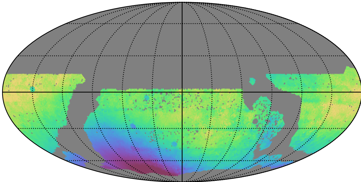
baseline_v3.3_10yrs WFD r band: Median solarElong
