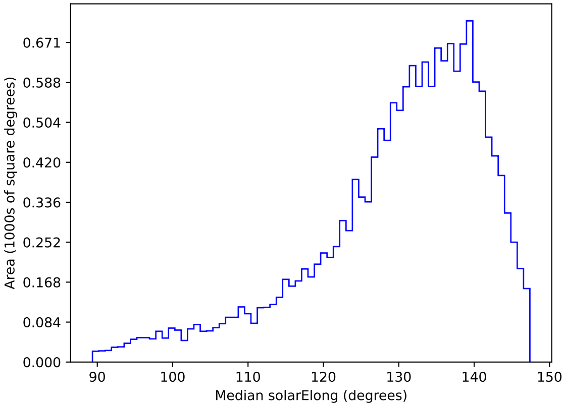
baseline_v3.3_10yrs WFD r band: Median solarElong
