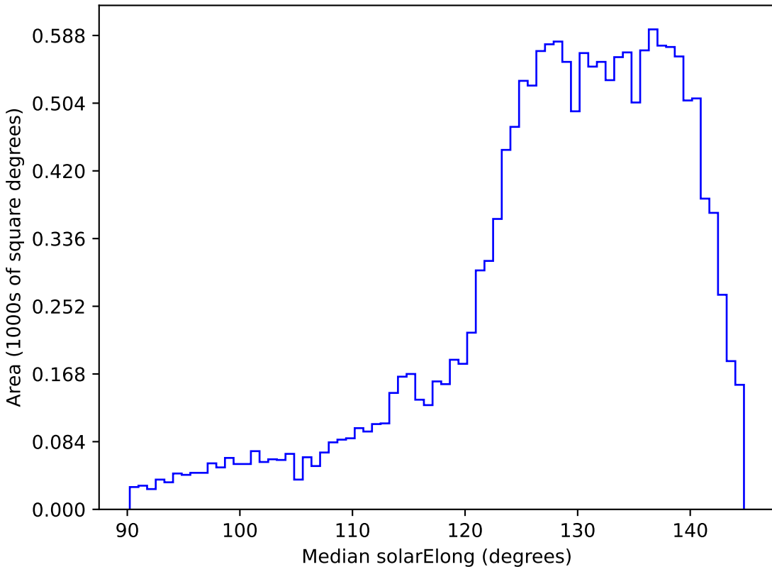
baseline_v3.3_10yrs WFD i band: Median solarElong
