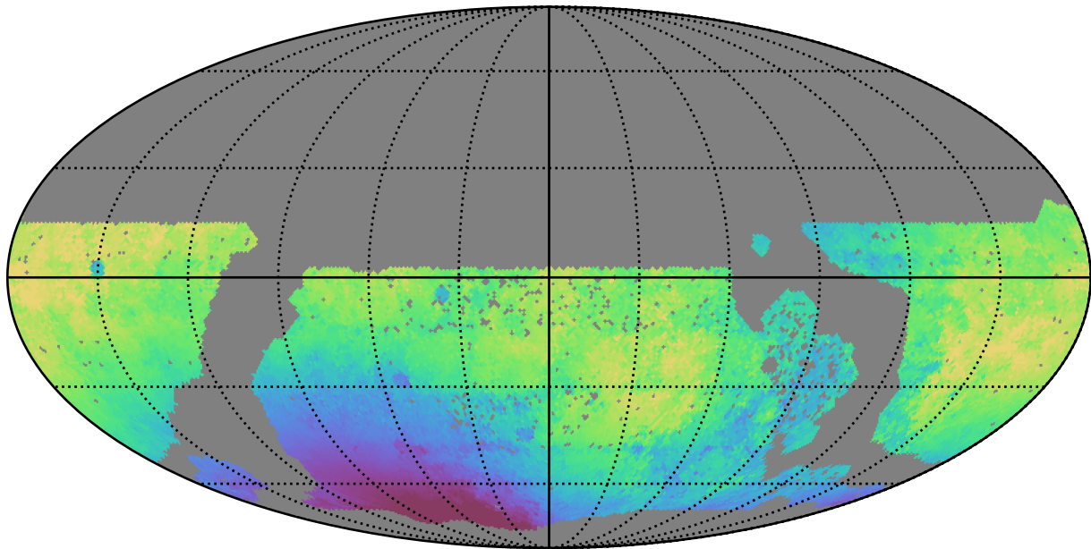
baseline_v3.3_10yrs WFD g band: Median solarElong
