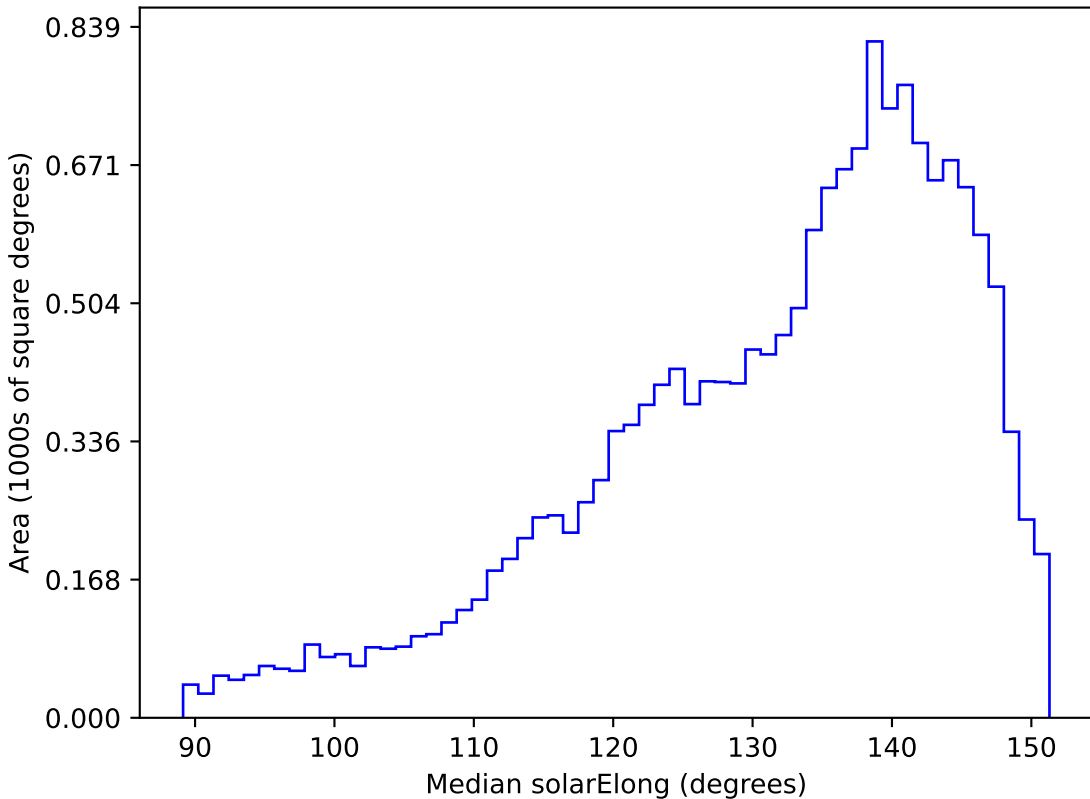
baseline_v3.3_10yrs WFD g band: Median solarElong
