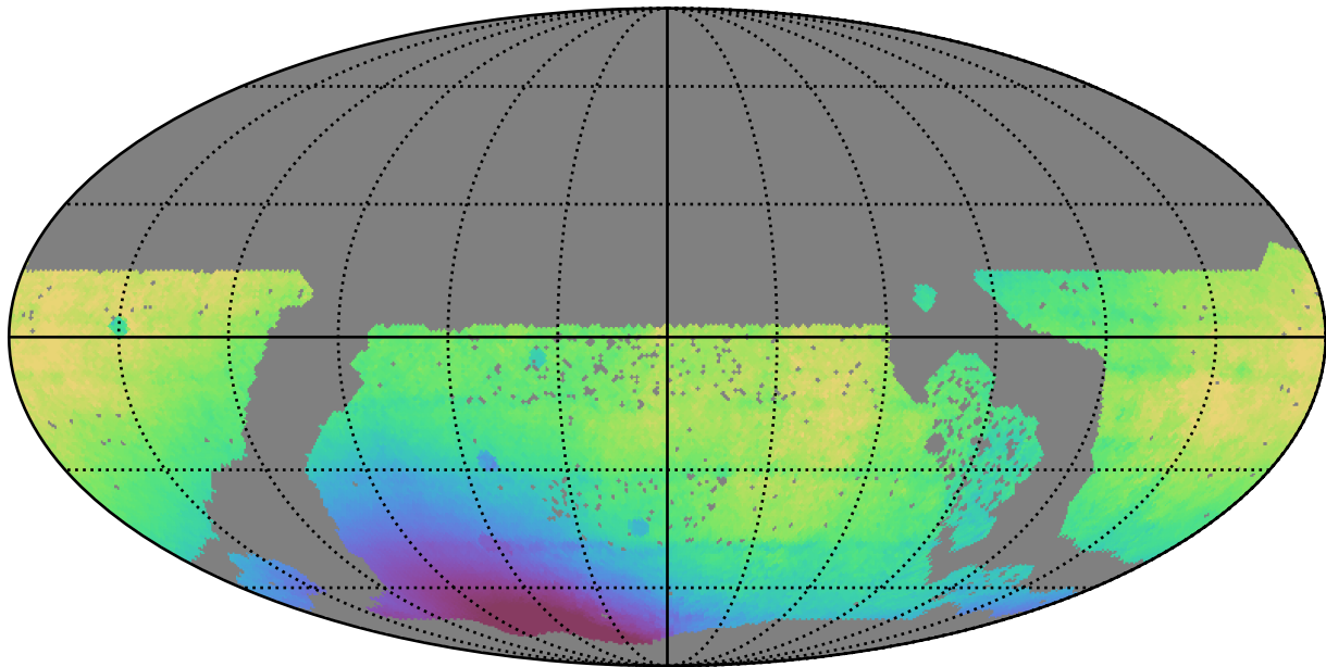
baseline_v3.3_10yrs WFD all bands: Median solarElong
