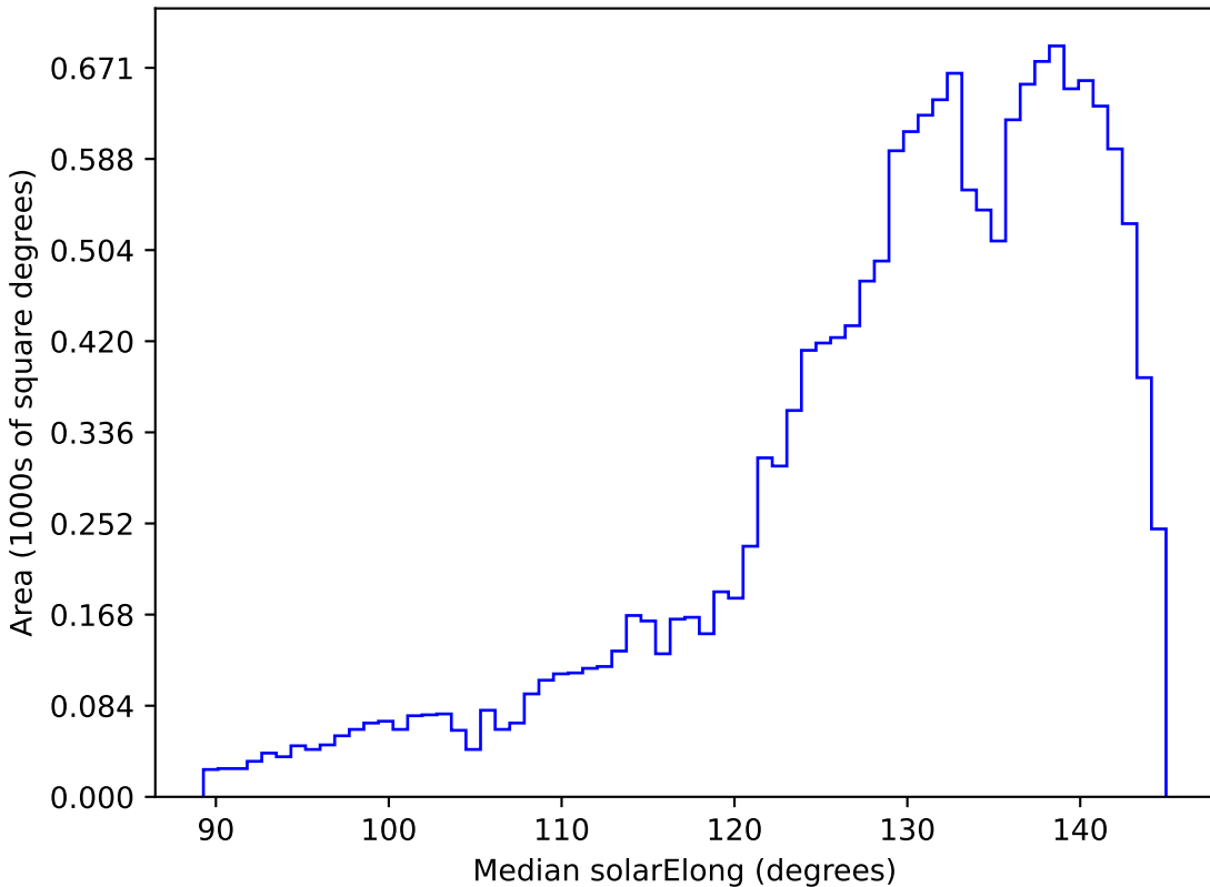
baseline_v3.3_10yrs WFD all bands: Median solarElong
