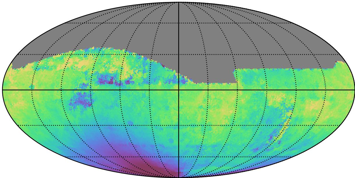
baseline_v3.3_10yrs All sky z band: Median solarElong
