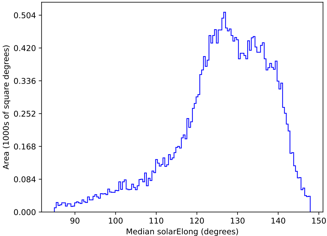
baseline_v3.3_10yrs All sky z band: Median solarElong
