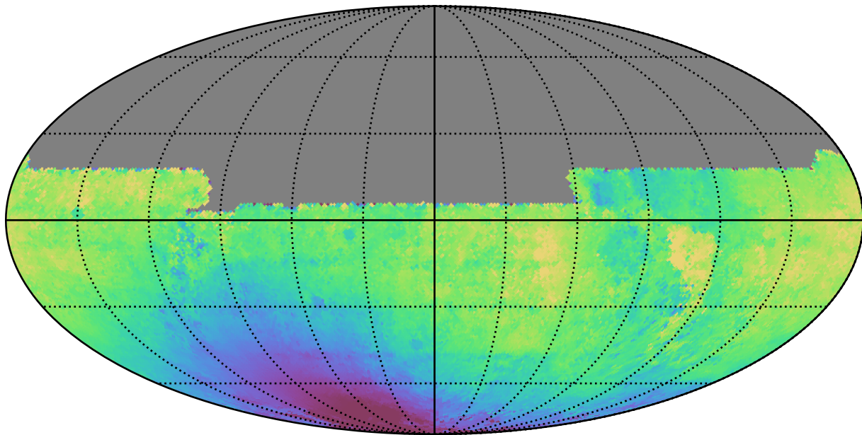
baseline_v3.3_10yrs All sky y band: Median solarElong
