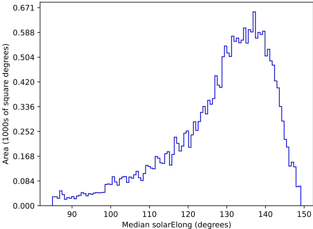
baseline_v3.3_10yrs All sky y band: Median solarElong
