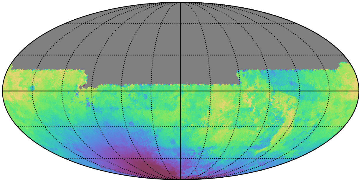
baseline_v3.3_10yrs All sky u band: Median solarElong
