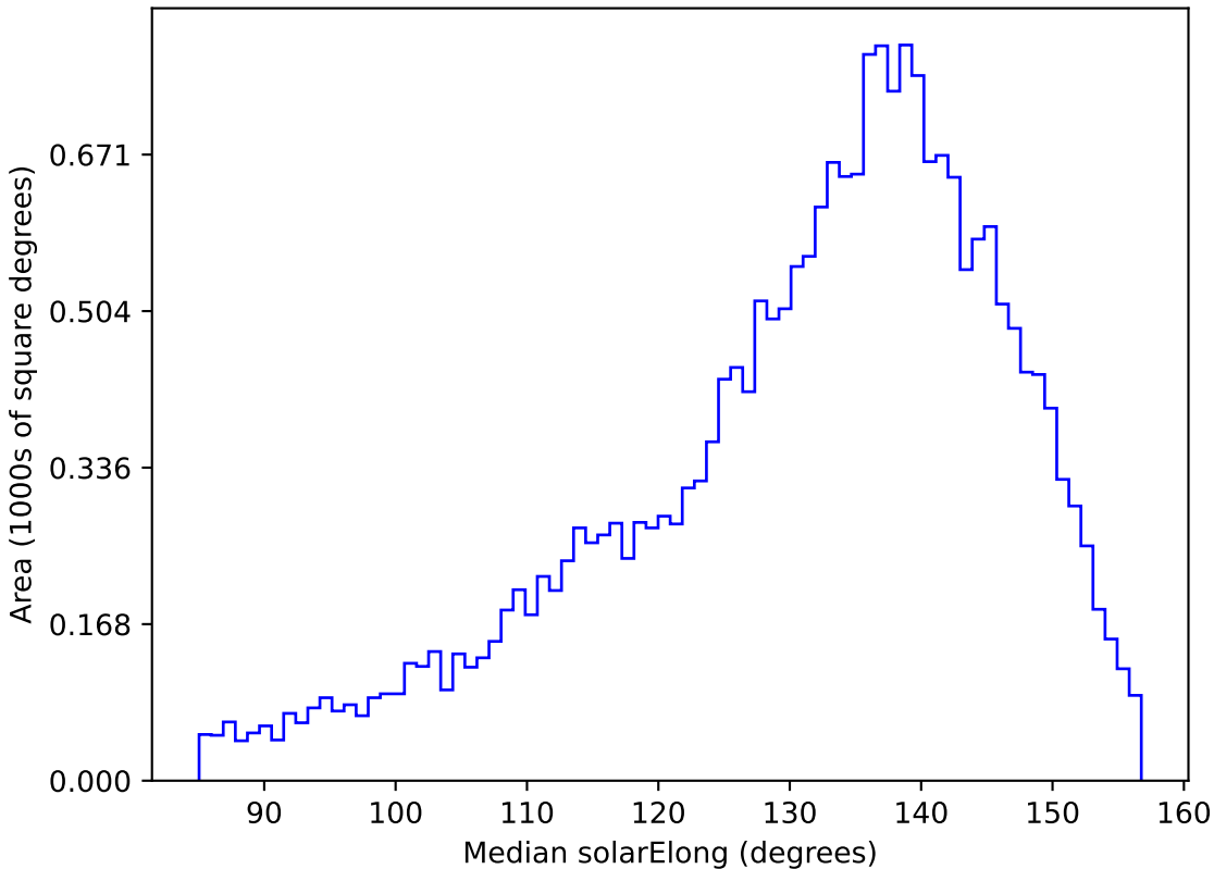
baseline_v3.3_10yrs All sky u band: Median solarElong
