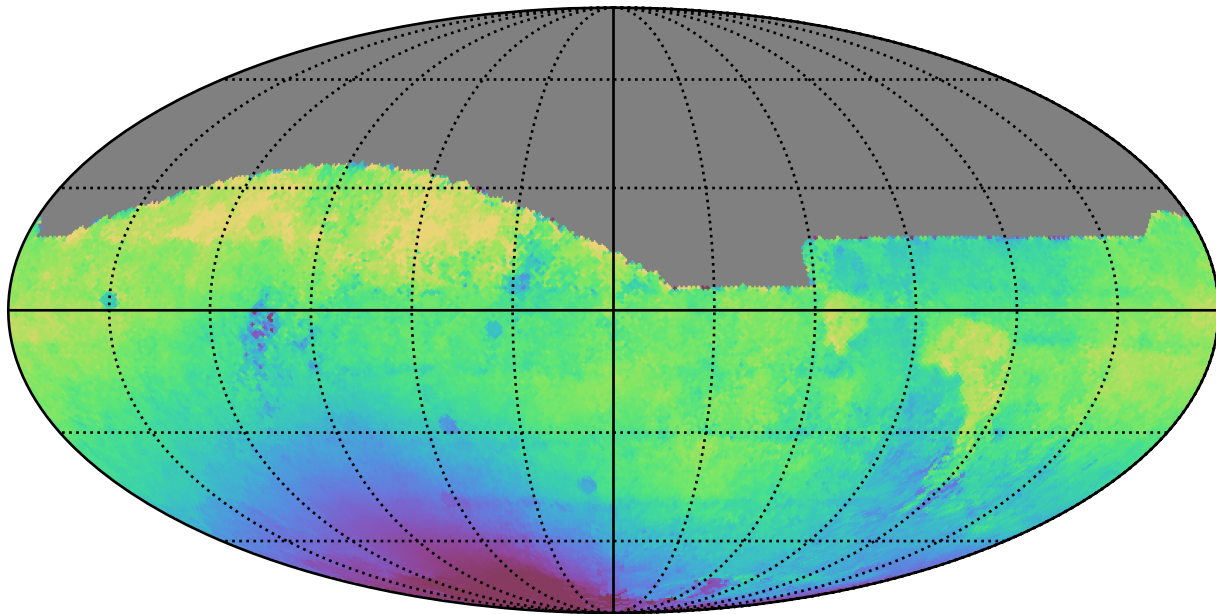
baseline_v3.3_10yrs All sky r band: Median solarElong
