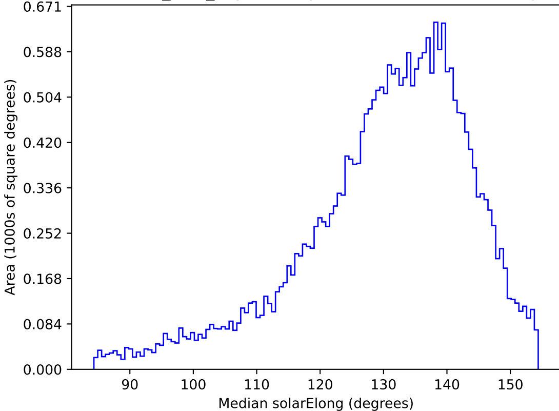
baseline_v3.3_10yrs All sky r band: Median solarElong
