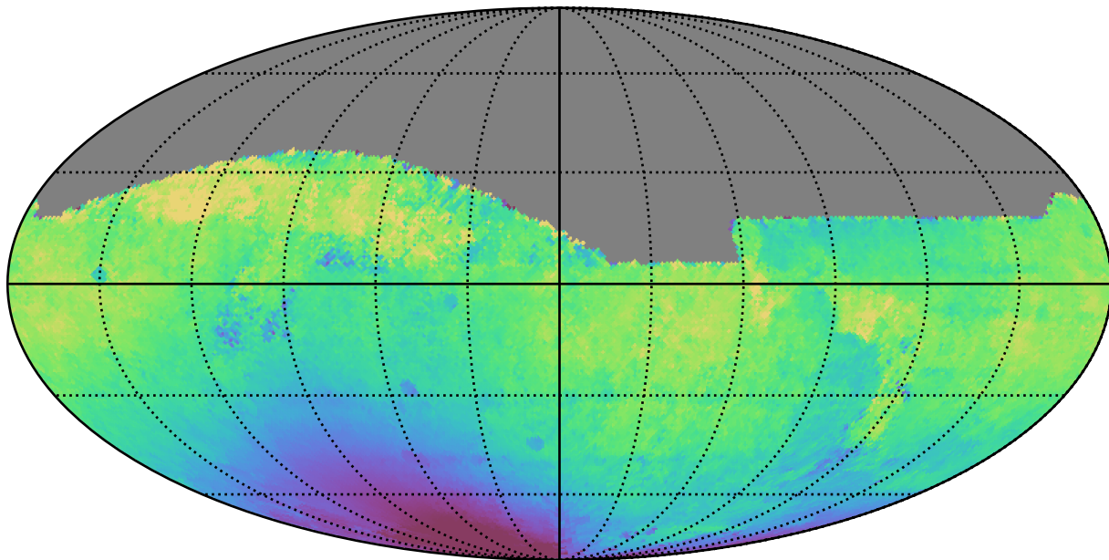
baseline_v3.3_10yrs All sky i band: Median solarElong
