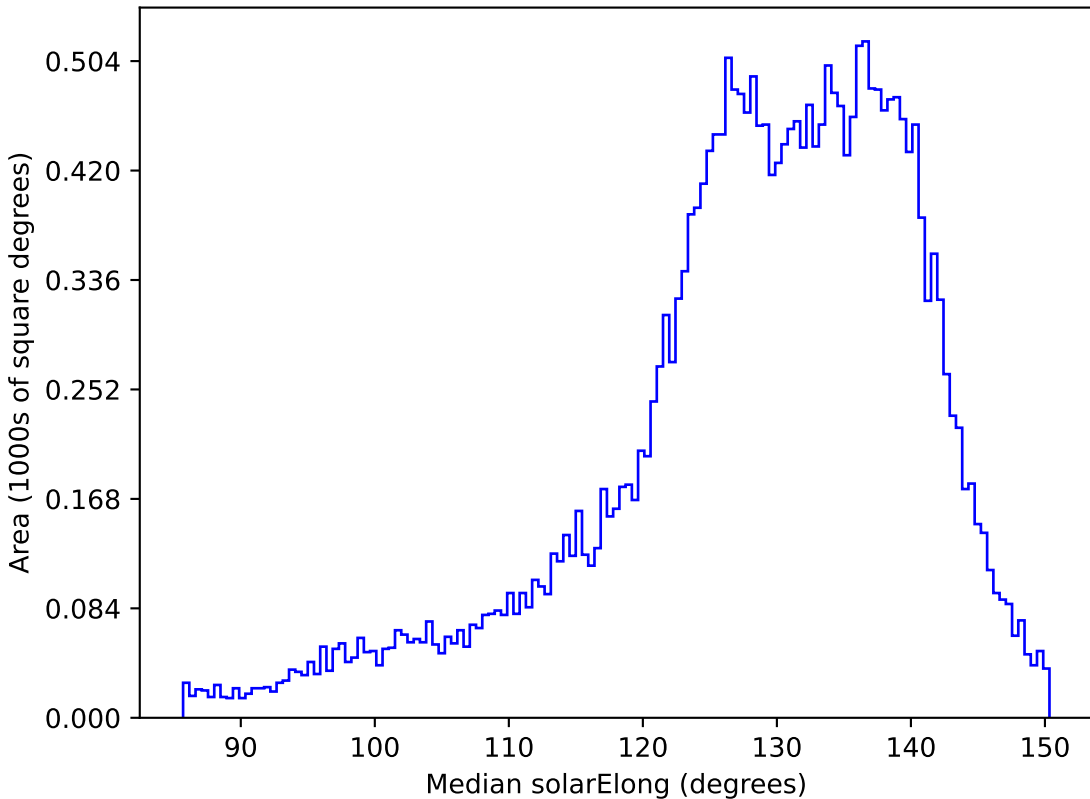
baseline_v3.3_10yrs All sky i band: Median solarElong
