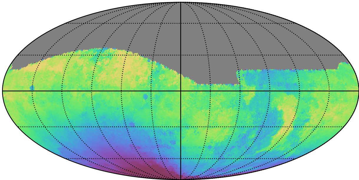
baseline_v3.3_10yrs All sky g band: Median solarElong
