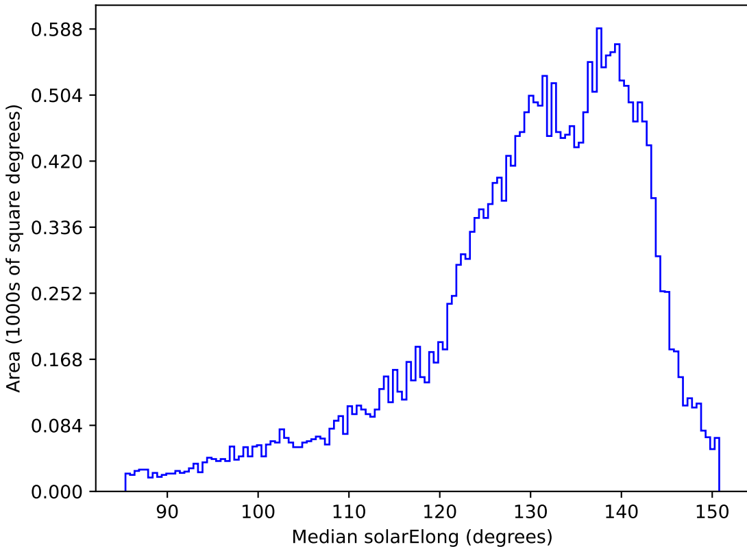
baseline_v3.3_10yrs All sky all bands: Median solarElong
